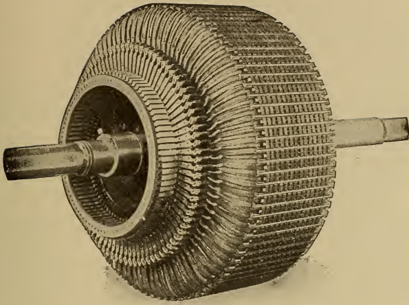
Fig. 11. ARMATURE COMPLETE. COMMUTATOR END.
